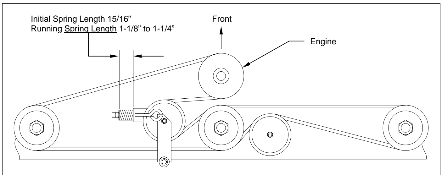
Figure 8: Belt Pattern and Spring Adjustment (Model H60T & H60H)
